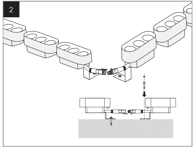
Fasten the screws to desire position & location.
