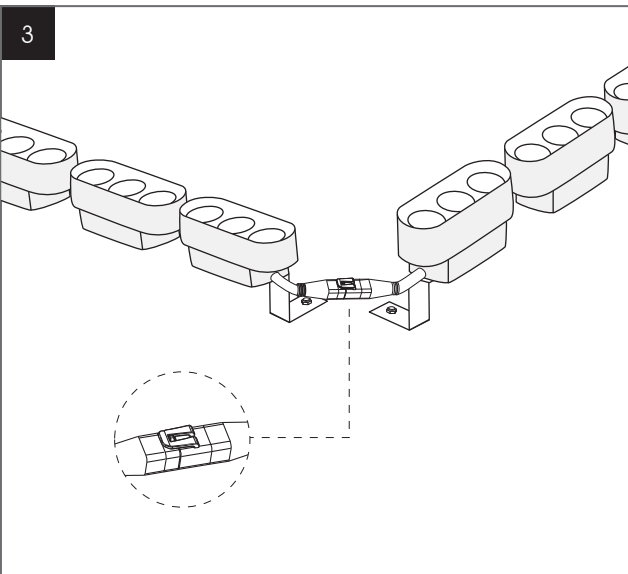
Connect male & female waterproof connector.
